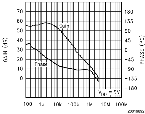
Open Loop Frequency Response, 5V
