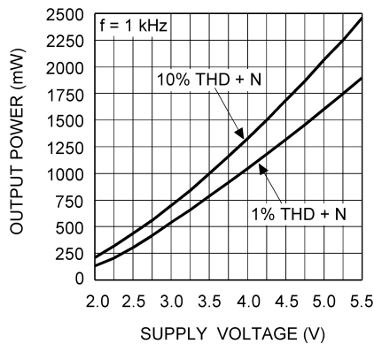
Output Power vs. Supply Voltage, 4Ω
