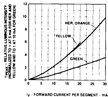
Figure 12. Relative Luminous Intensity vs. DC Forward Current.
