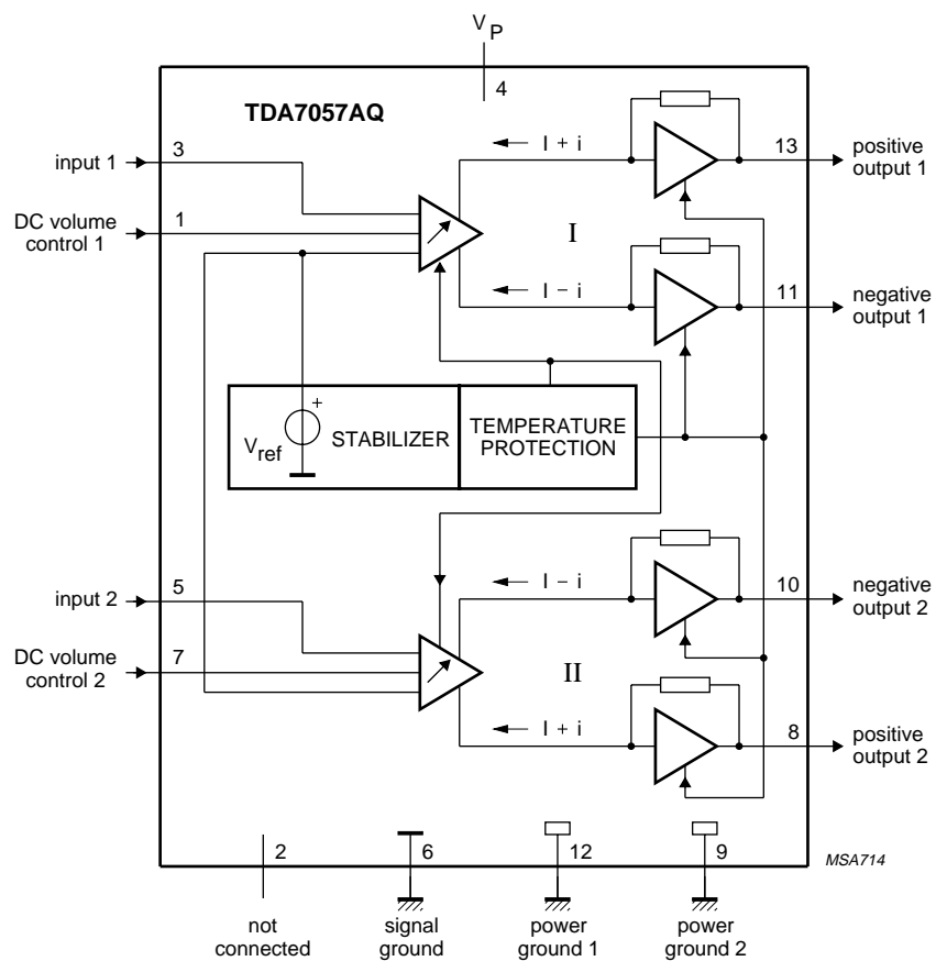
Fig.1 Block diagram.
