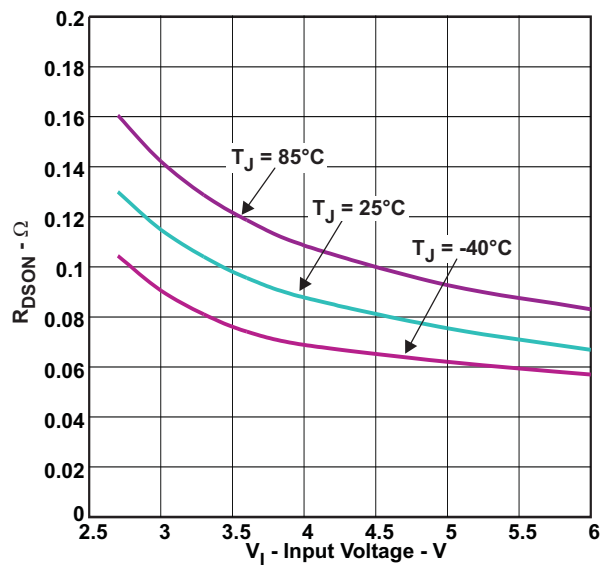
Figure 11. High-Side Switch
