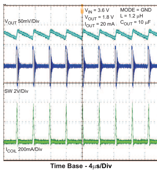
Figure 14. Typical Operation (PFM Mode)
