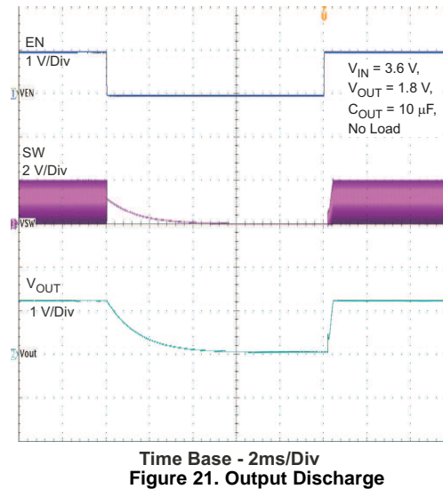
Figure 21. Output Discharge
