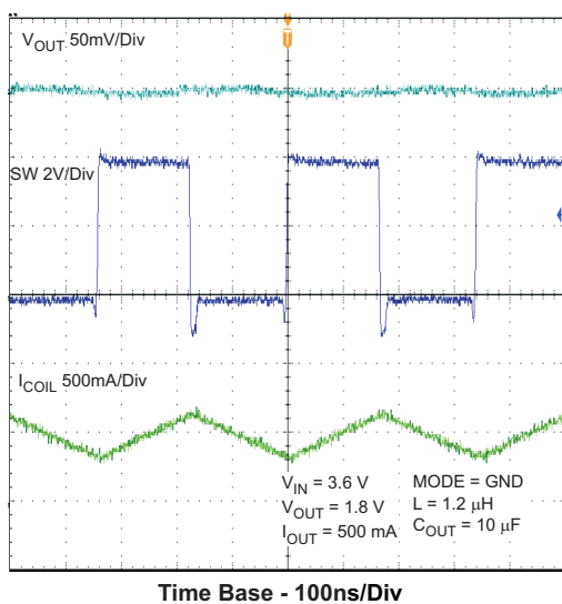
Figure 13. Typical Operation (PWM Mode)
