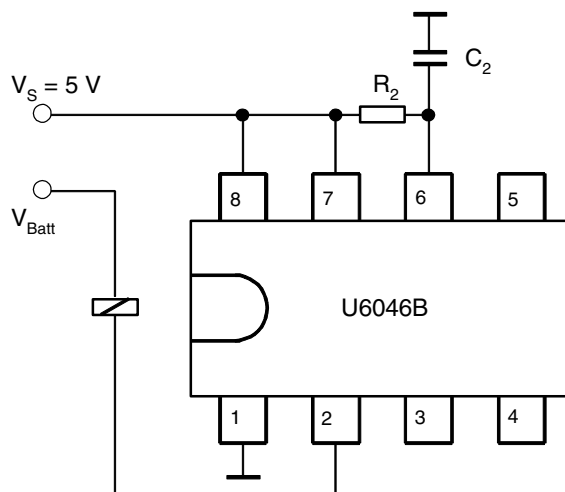
Figure 4. Basic Circuit for V_S = 5 \text{ V}
