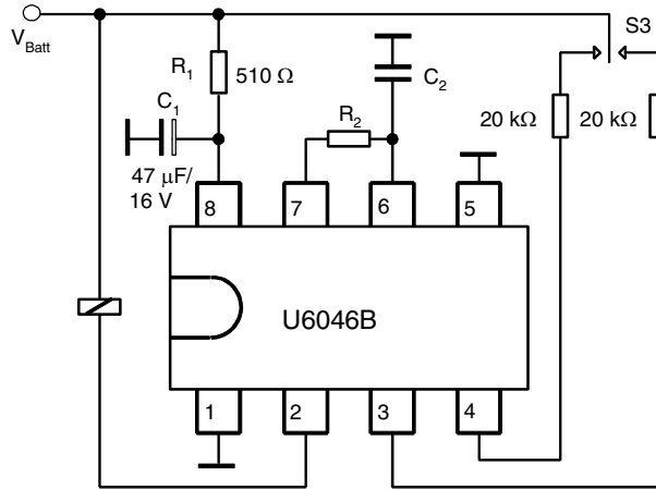
Figure 6. ON/OFF Function
