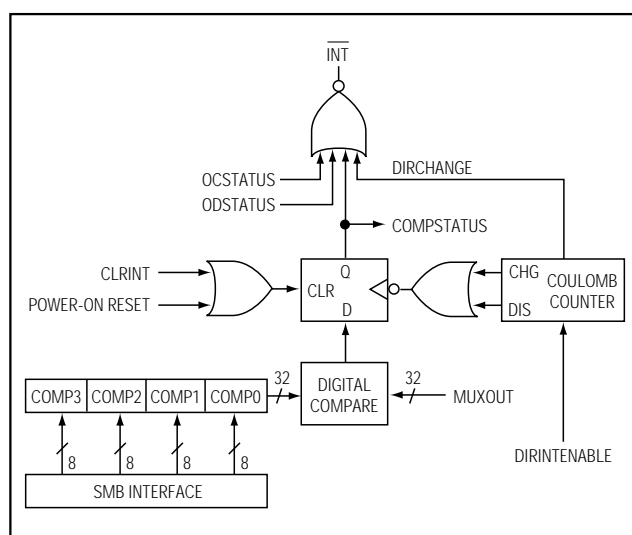
Figure 5. Digital Compare Section Functional Diagram
