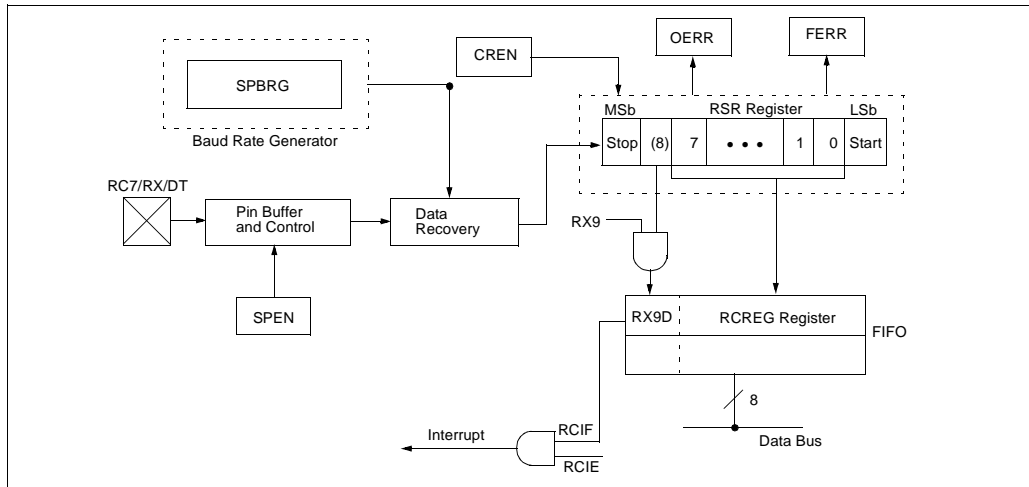
FIGURE 11-5: ASYNCHRONOUS RECEPTION
