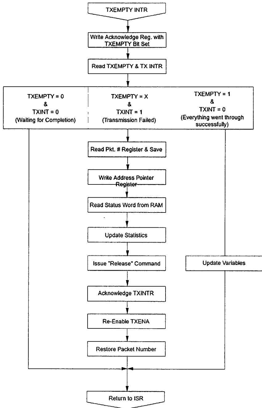
FIGURE 15 - TXEMPTY INTR (Assumes Auto Release Option Selected)
