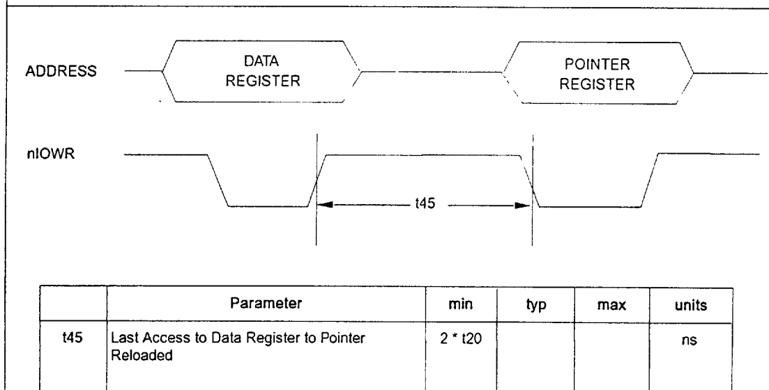
FIGURE 42 - MEMORY READ TIMING
