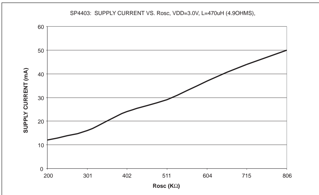
Figure 8. I_{TOTAL} vs R_{OSC} , V_{DD}=3.0V , Coil=470\mu H , 4.9Ω
