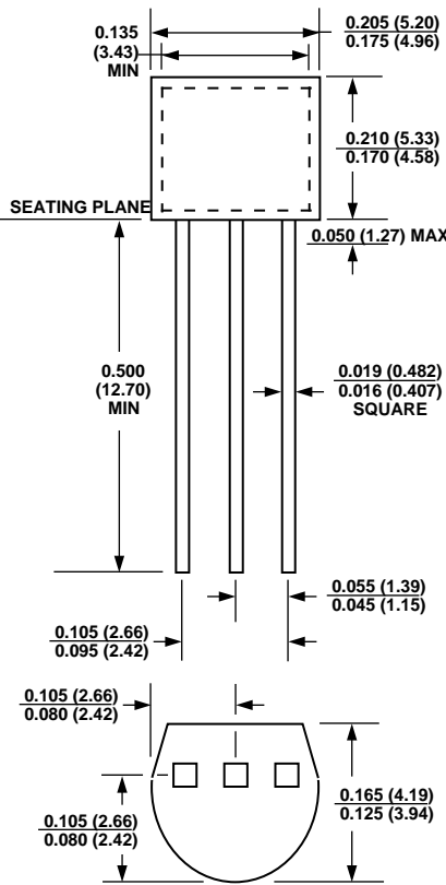
3-Pin TO-92
